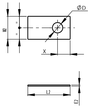
Plaquettes type J J Locking Plates
